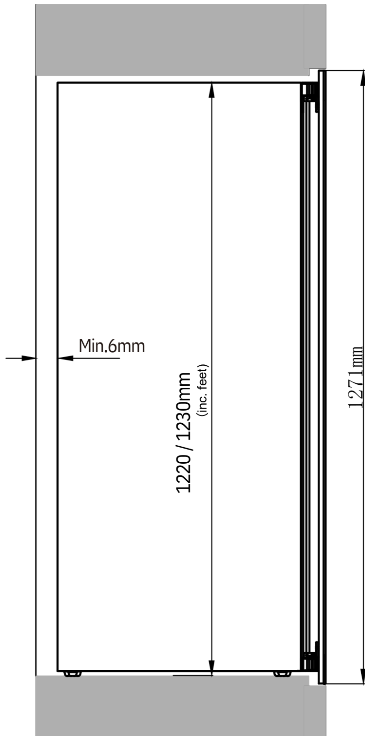
Side View
